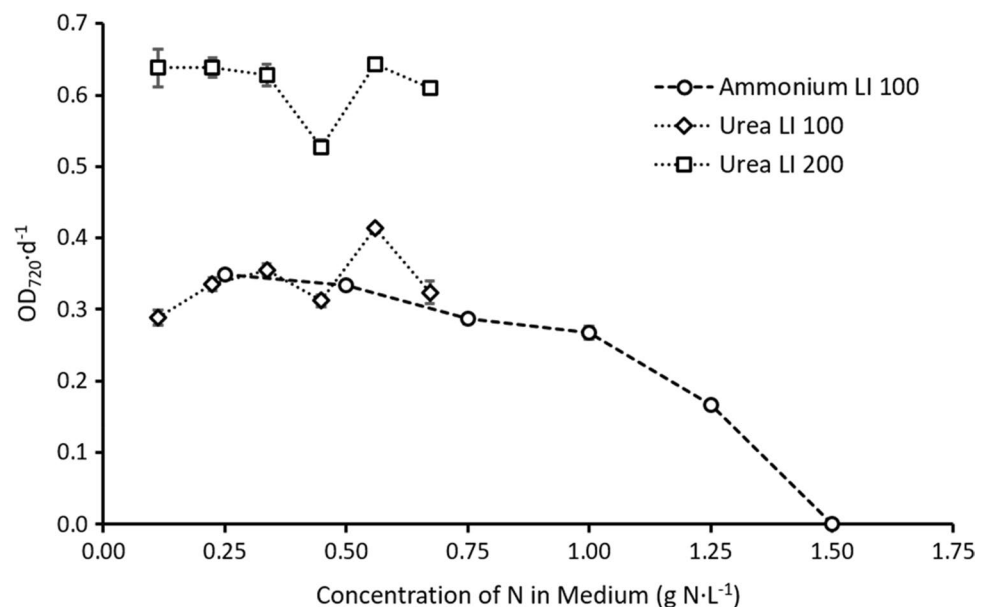
Fig. 2 Growth rate ( OD_{720} \text{ day}^{-1} ) during the linear growth phase of Synechocystis 6803 cultivated on modified BG11 with increasing concentrations of \text{NH}_4^+\text{-N} or Urea-N at a pH of 7.5 at a temperature of 35^\circ\text{C} and under a light intensity (LI) of 100 or 200 \mu\text{mol photons m}^{-2} \text{ s}^{-1} . Averaged values determined by linear regression ( R^2=0.99 ). Error bars are the standard deviation of four replicates and are covered by the marker if not visible
