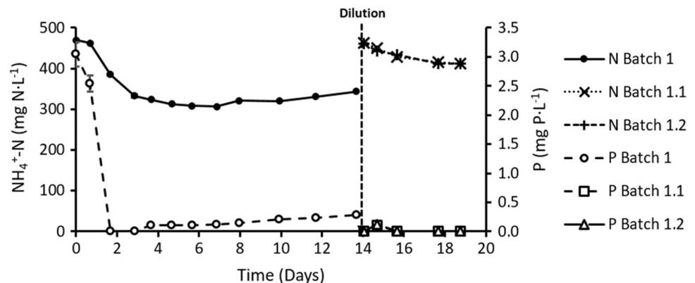
Fig. 5 \text{NH}_4^+\text{-N} concentration in medium during cultivation of Synechocystis 6803 under phosphorus-limiting conditions, at a pH of 7.5, a temperature of 35 \text{ }^\circ\text{C} , and under a light intensity of 600 \mu\text{mol photons m}^{-2} \text{ s}^{-1} . Error bars are the standard deviation of samples taken in duplicate and are covered by the marker if not visible
